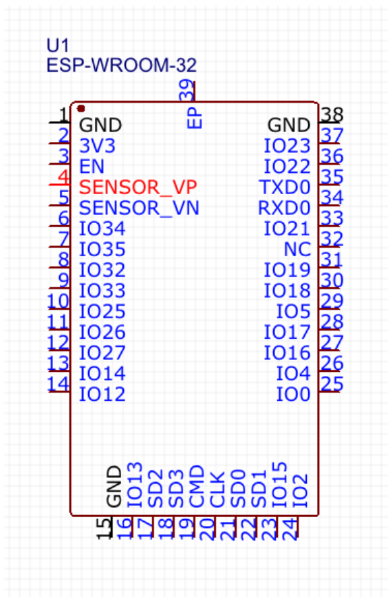
Figure 6: ESP32 Pin Layout
